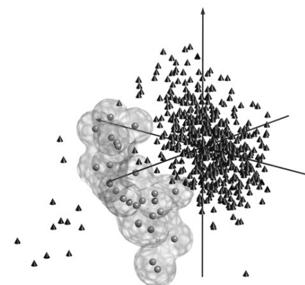
Fig.2: Three dimensional illustration of 548 spectral data points. TAD Salmonella vac® E data points are depicted as light grey balls, others as black cones. The three dimensions of the illustration correspond to three chosen components from a principal component analysis of all spectra. Using these three components, VAC E is clearly distinguishable from its vicinity. For further clarification of separability, the space around the data points is denoted by a virtual surface.
