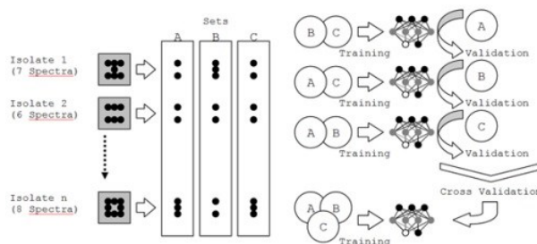
Fig.1: Stratified set formation and cross validation. Spectra of each isolate were evenly divided into three groups. Subsequent cross validation was performed in three rounds. In each round, two groups of spectra were used for training of an artificial neural network (ANN) with the object of being able to differentiate vaccine from non-vaccine strains. The outcome of this learning process was examined using the third group (validation). The combined validation result of all three rounds yielded the so-called cross validation. This served to assess the quality of an ANN which was subsequently trained with all spectra simultaneously.
